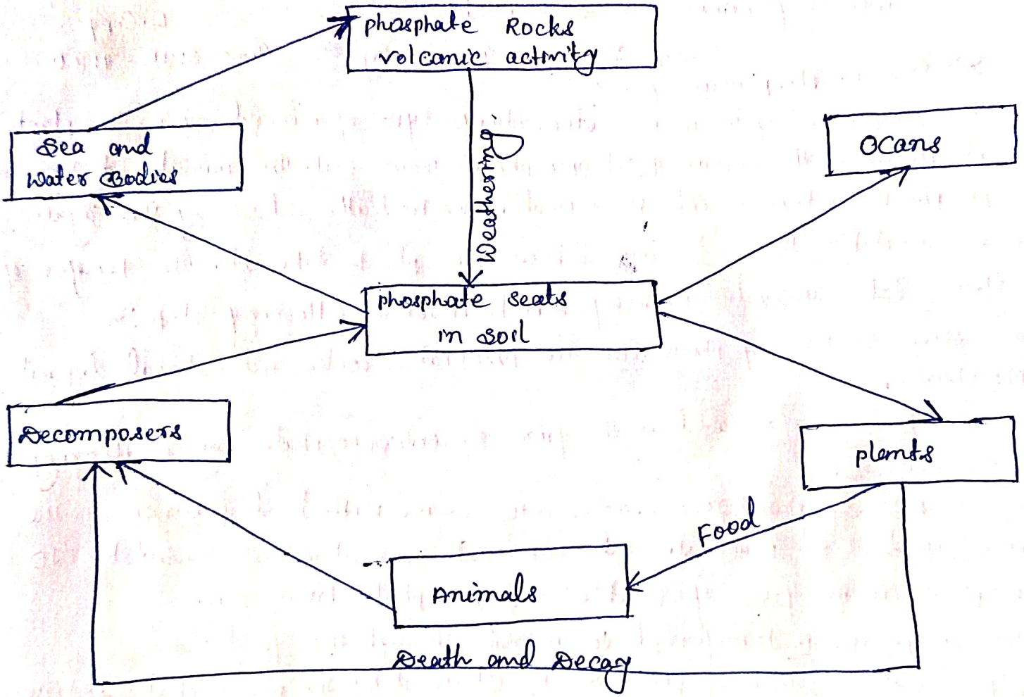
Fig - phosphorus cycle.
